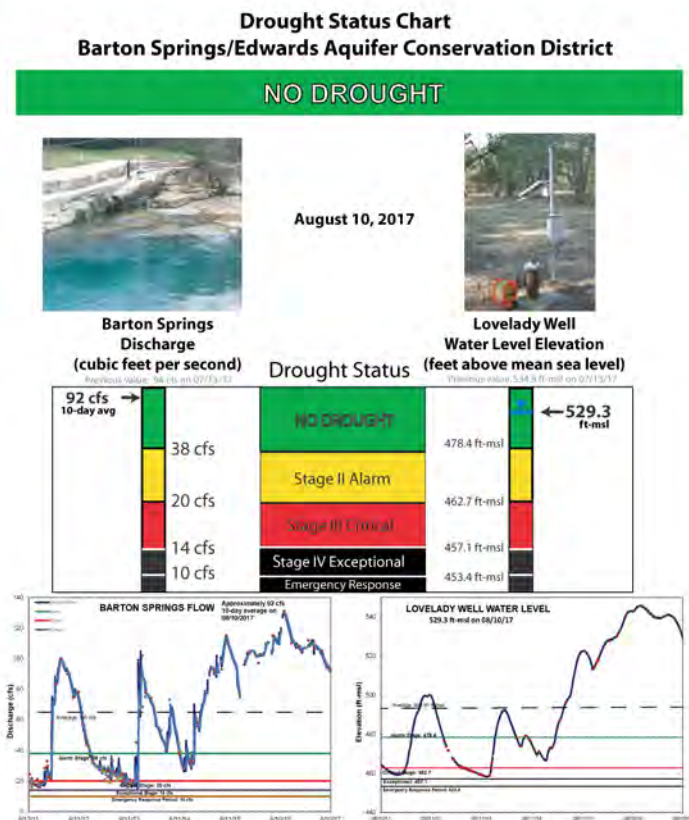
Figure 4. Drought status chart showing indices and thresholds for drought declarations made by the Board of Directors of the District.
