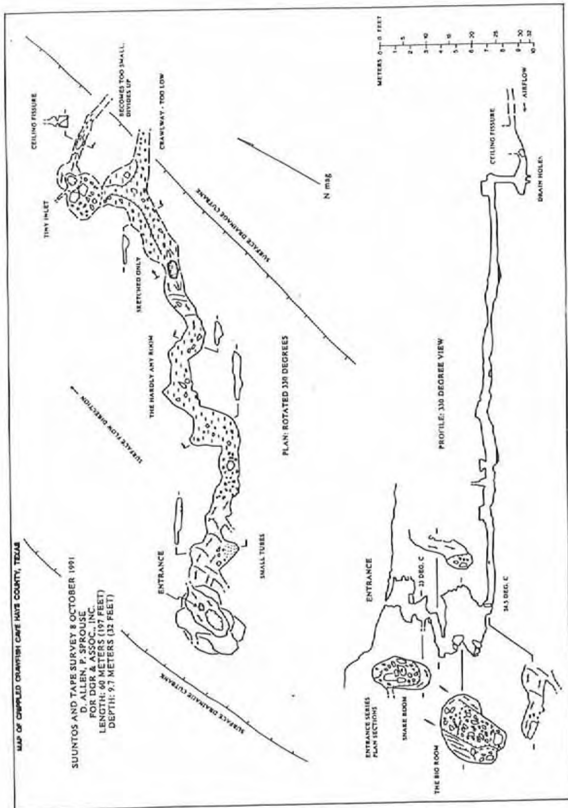
Map of Crippled Crawfish Cave, Hays County, Texas
